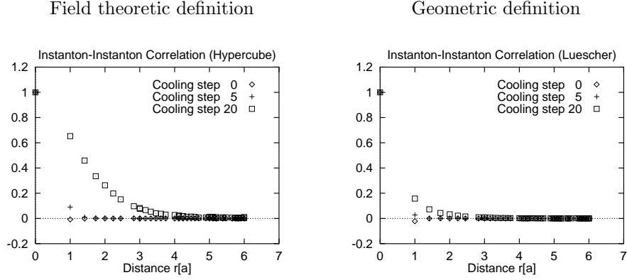
Figure 1. Auto-correlation functions of the topological charge density using the hypercube definition (l.h.s.) and the Lüscher definition (r.h.s.) in the confinement phase for 0, 5, 20 cooling steps. Both auto-correlations grow with cooling indicating the existence of extended instantons.
